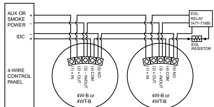
Figure 3b: Wiring Diagram, 4W-B and 4WT-B
